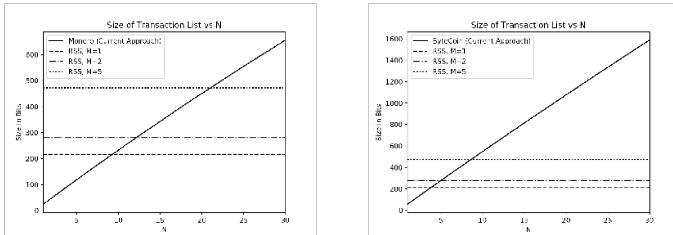
Fig. 3. Size of the transaction list \mathcal{T} in bits for two popular cryptocurrencies, Monero (left) and ByteCoin (right). “Current approach” indicates the representation of the transaction list as a function of N (the number of transactions on the list). Note that this value is (mostly) independent of M , so we do not illustrate different values of M . “RSS” indicates the cost of the compact description W for different values of M , N . For ByteCoin we use \ell = 2,000,000 and for Monero we use \ell = 4,000,000 .
