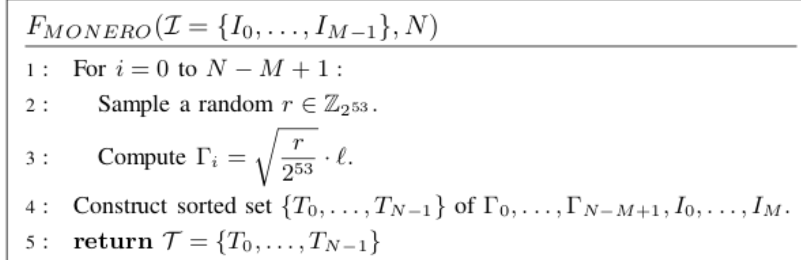
Fig. 2. Monero sampling technique
