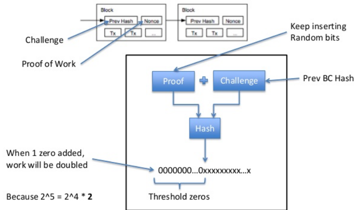
Figure 2: Proof-of-work
