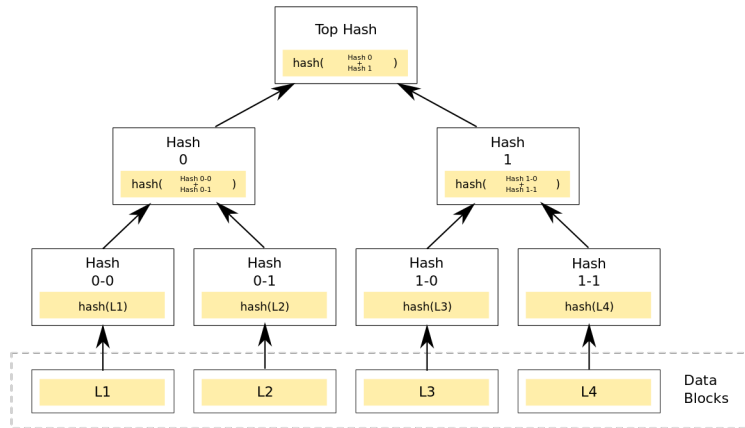
Figure 1: Merkle Tree
